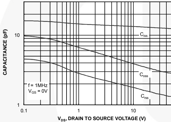
Figure 9. Capacitance Characteristics
