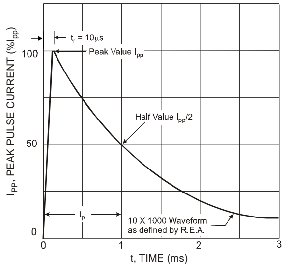
Figure 4. Pulse Waveform
