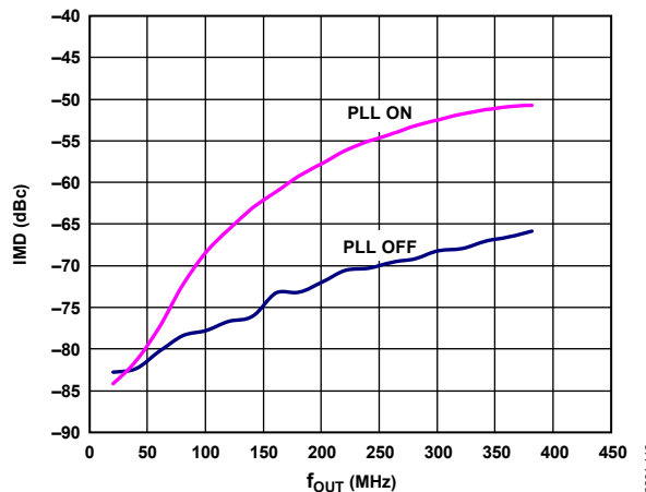
Figure 21. IMD vs. f_{OUT} , 4× Interpolation, f_{DATA} = 200 MSPS, Digital Scale = 0 dBFS, I_{FS} = 20 mA, PLL On and PLL Off
