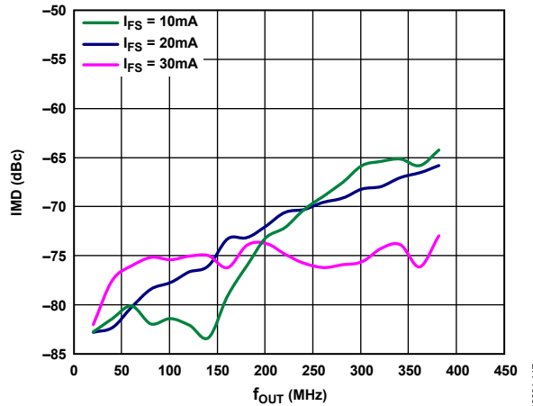
Figure 20. IMD vs. f_{OUT} over I_{FS} , 2× Interpolation, f_{DATA} = 400 MSPS, Digital Scale = 0 dBFS
