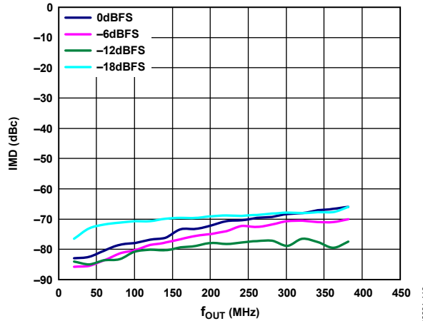
Figure 19. IMD vs. f_{OUT} over Digital Scale, 2× Interpolation, f_{DATA} = 400 MSPS, I_{FS} = 20 mA
