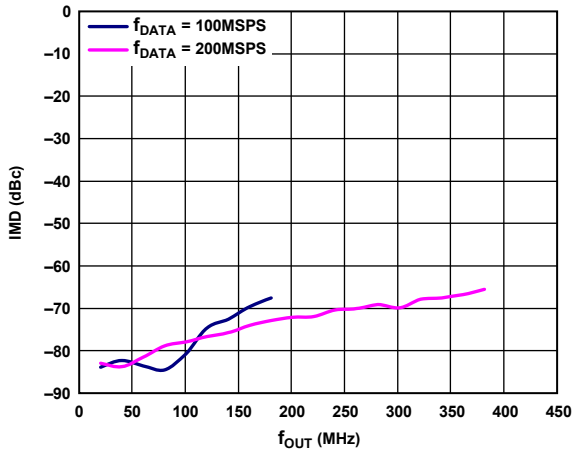
Figure 17. IMD vs. f_{OUT} over f_{DATA} , 4× Interpolation, Digital Scale = 0 dBFS, I_{FS} = 20 mA
