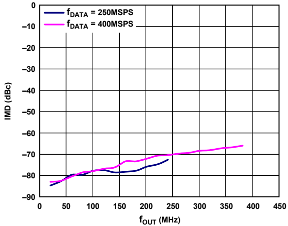
Figure 16. IMD vs. f_{OUT} over f_{DATA} , 2× Interpolation, Digital Scale = 0 dBFS, I_{FS} = 20 mA
