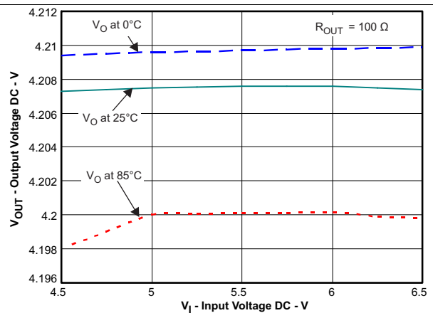
Figure 2. Line Regulation
