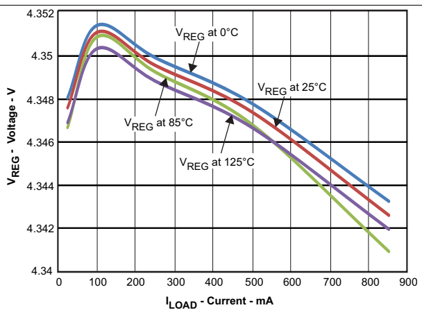
Figure 4. Load Regulation
