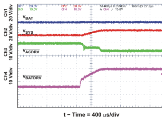
Figure 20. System Selector On Adapter Removal With 390 µF SYS-to-PGND System Capacitor
