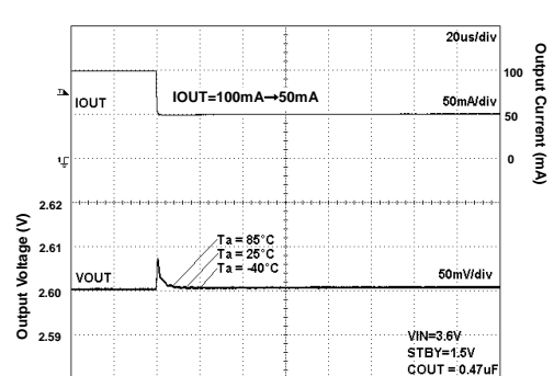
Fig 148. Load Response
