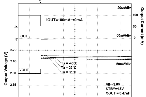
Fig 144. Load Response
