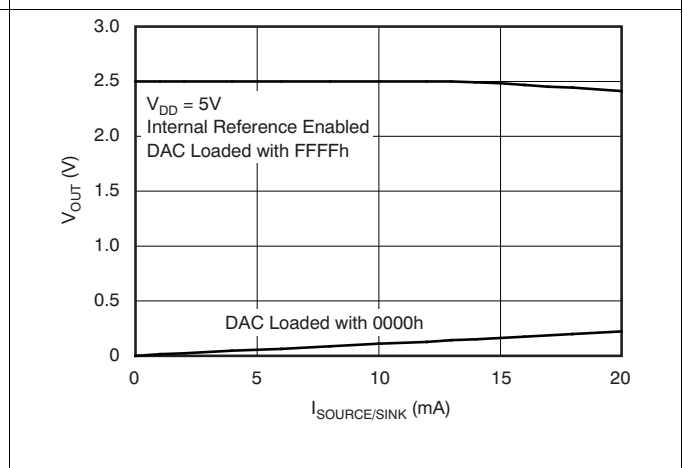
Figure 19. Source and Sink Current Capability
