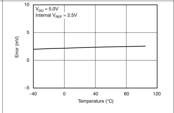
Figure 17. Zero-Scale Error vs Temperature
