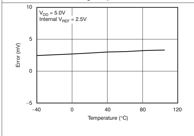
Figure 18. Full-Scale Error vs Temperature
