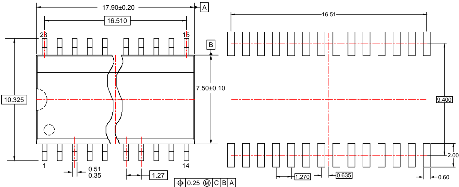
TOP VIEW
