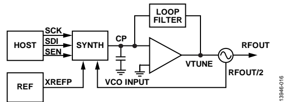
Figure 16. Typical Application Diagram
