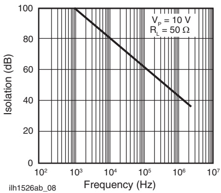
Fig. 9 - Output Isolation
