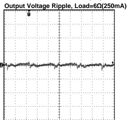
CH2: V_{OUT} , C_{OUT} = 4.7\mu F ; Scale: 20mV/Div, AC Coupled Time scale: 200ns/Div
