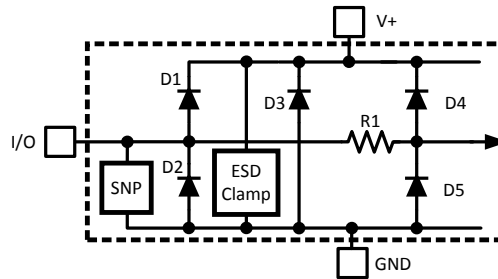
Figure 3. ESD Protection Input Structure
