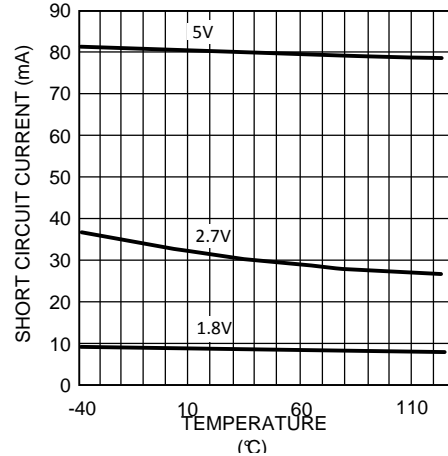
Figure 28. Short Circuit Current vs Temperature (Sourcing)
