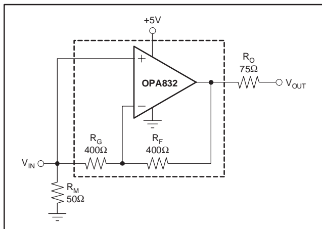
Figure 7. Improved Unity-Gain Buffer
