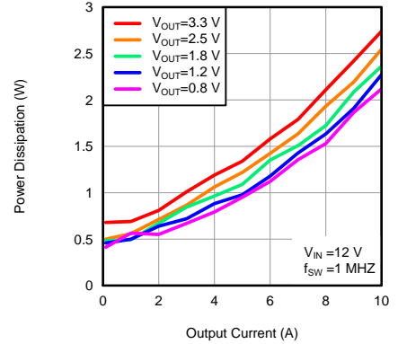
Figure 6. Power Dissipation
