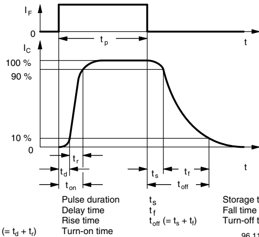
Fig. 3 - Switching Times
