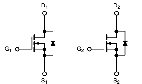
N-Channel MOSFET
