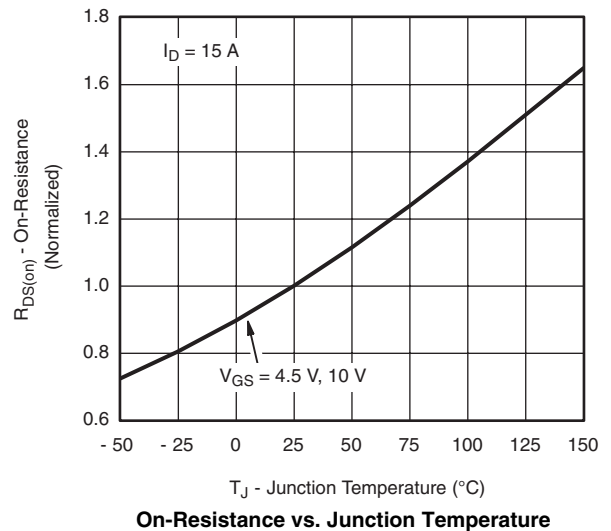
I_D = 15\text{ A} V_{GS} = 4.5\text{ V}, 10\text{ V} On-Resistance vs. Junction Temperature
