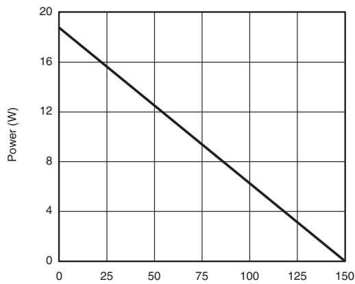
Power Derating, Junction-to-Case
