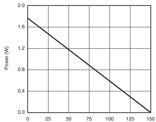
Power Derating, Junction-to-Ambient
