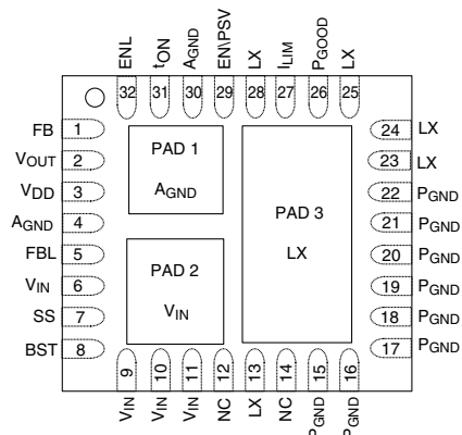
SiC401A/B Pin Configuration (Top View)
