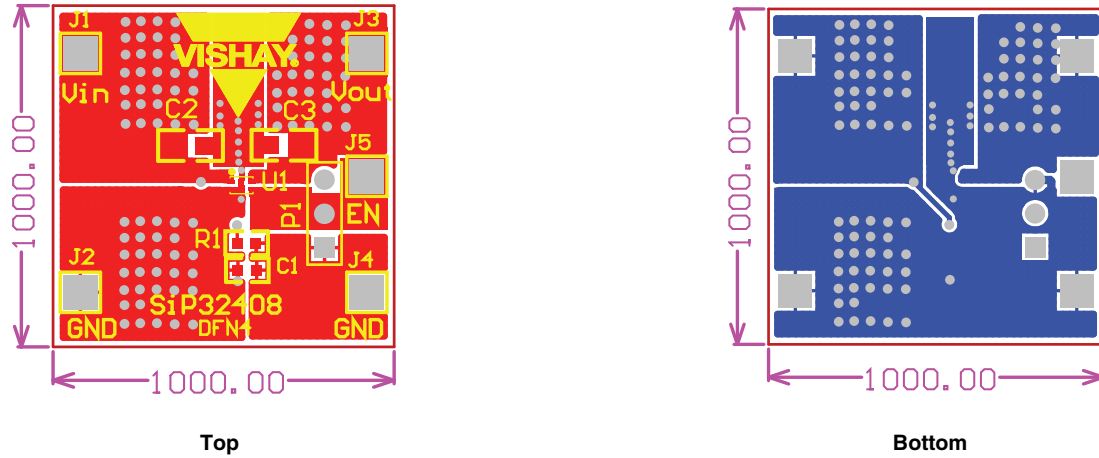
Figure 29 - Evaluation board Layout for TDFN4 1.2 mm x 1.6 mm (type: FR4, size: 1" x 1", thickness: 0.062", copper thickness: 2 oz.)
