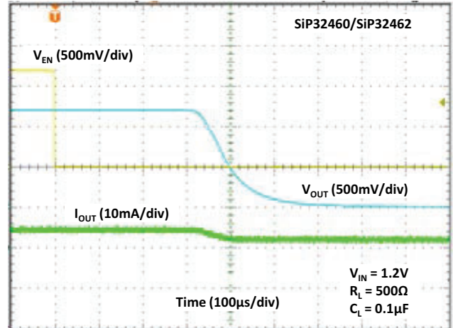
Fig. 35 - Turn-off Time
