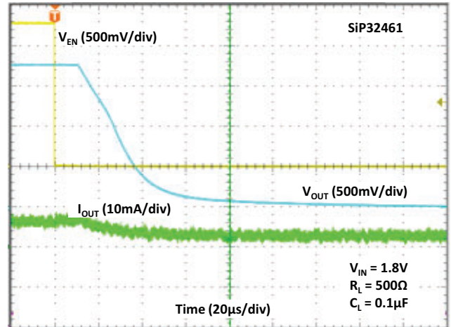
Fig. 41 - Turn-off Time
