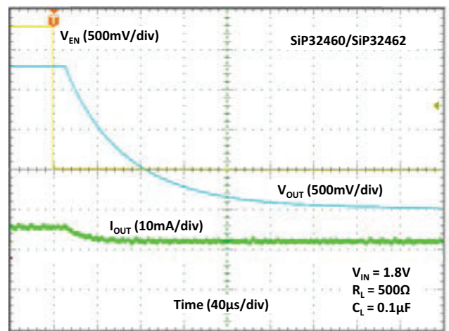
Fig. 36 - Turn-off Time
