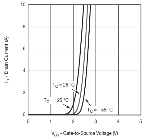
Transfer Characteristics
