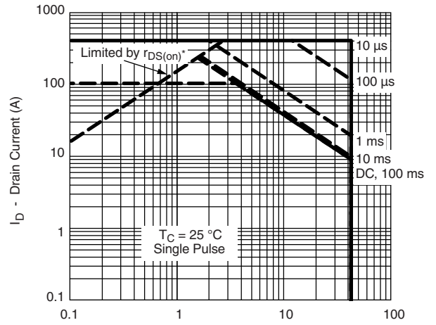
Safe Operating Area T_C = 25\text{ }^\circ\text{C} Single Pulse * V_{GS} > minimum V_{GS} at which r_{DS(on)} is specified
