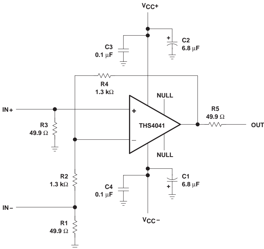
Figure 76. THS4041 Evaluation Board
