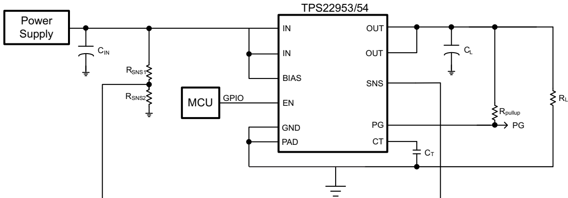
Figure 62. Monitoring The Input Voltage Schematic
