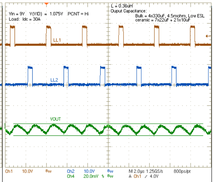
Figure 31. Output Ripple, V_{IN} = 9V
