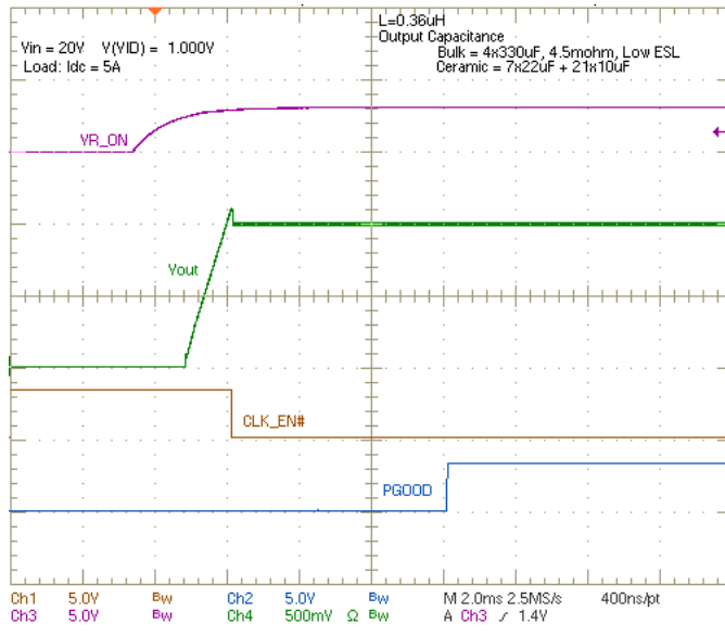
Figure 28. \overline{PG} and PGOOD, V_{IN} = 20V
