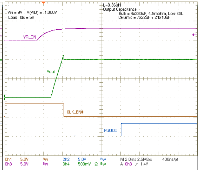
Figure 29. \overline{PG} and PGOOD, V_{IN} = 9V
