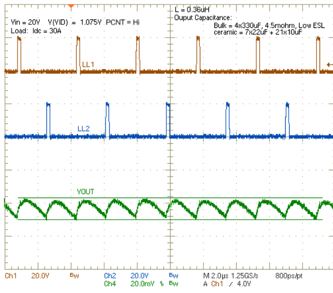
Figure 30. Output Ripple, V_{IN} = 20V
