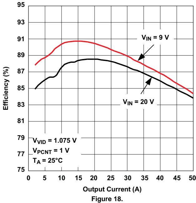
HIGH FREQUENCY MODE (HFM) EFFICIENCY vs OUTPUT CURRENT
