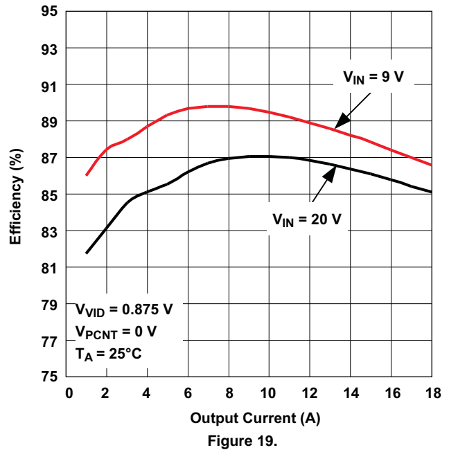
LOW FREQUENCY MODE (LFM) EFFICIENCY vs OUTPUT CURRENT
