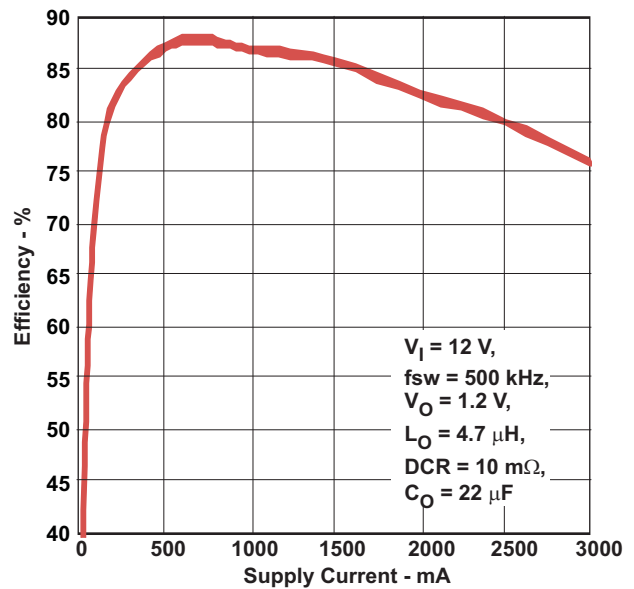
Figure 4. Buck 1 Efficiency, V_O = 1.2\text{ V} , V_{IN} = 12\text{ V} , f_{SW} = 500\text{ kHz} , L_O = 4.7\ \mu\text{H} , \text{DCR} = 10\ \text{m}\Omega , C_O = 22\ \mu\text{F}
