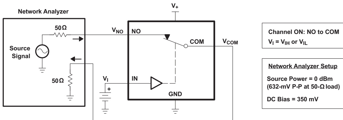
Figure 16. Bandwidth (BW)
