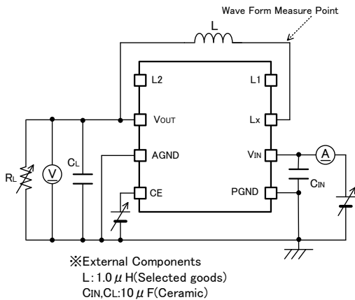
< Circuit No.① >
