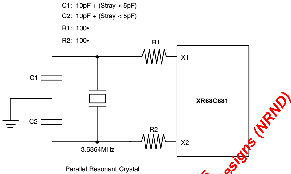
Figure 6. A Recommended Schematic for the XTAL Oscillator Circuitry
